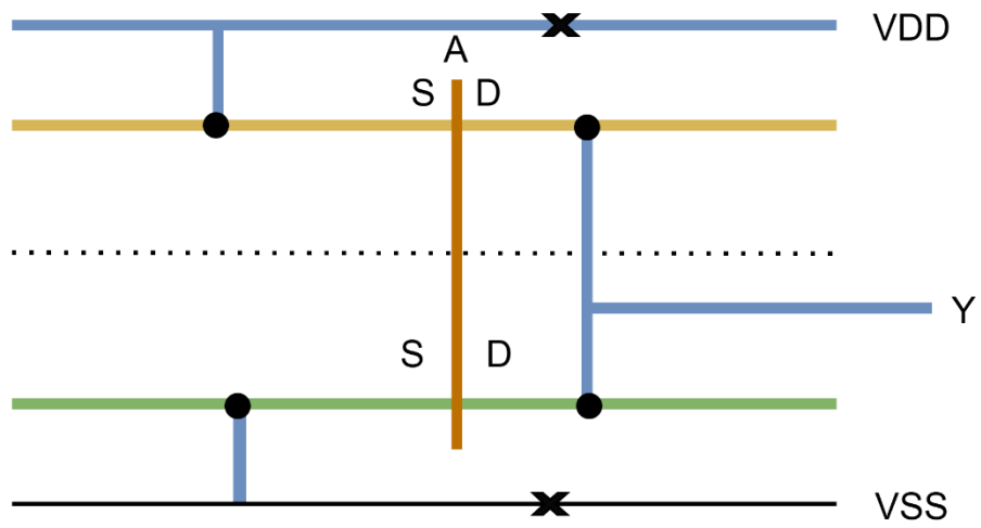
Inverter Stick Diagram
